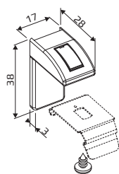
Fixing bracket
