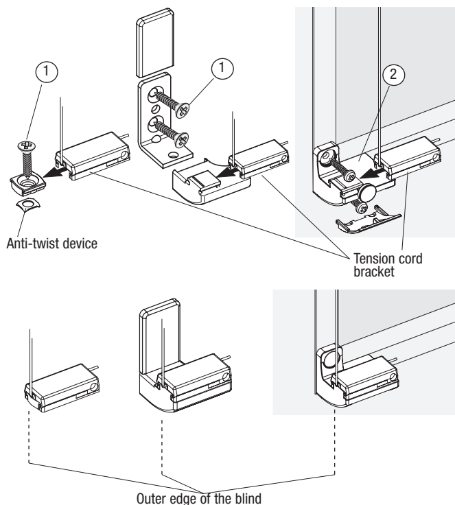
Holding brackets
